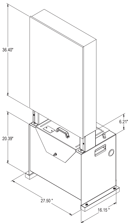
PLC Controller Tank
