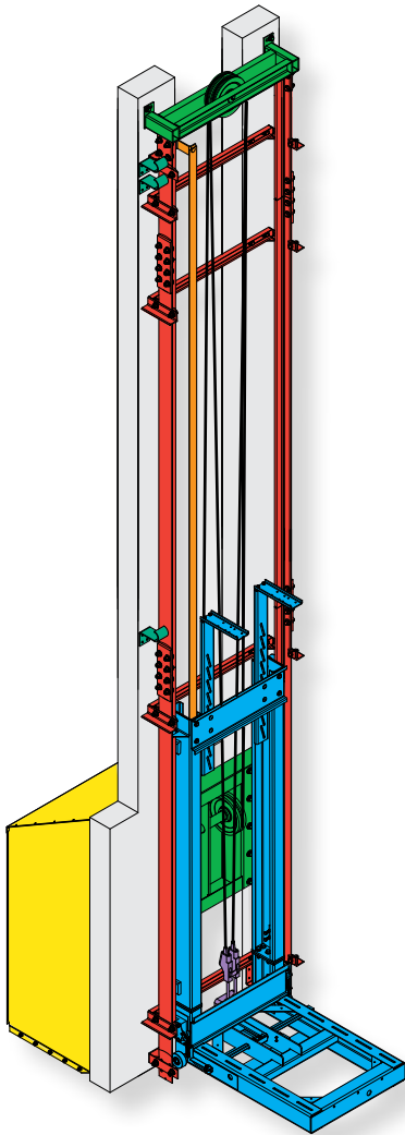
Excelelevator-RMR, Reduced Machine Room Winding Drum - Series 022 - Capacity 1,000 lbs
