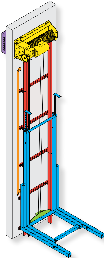
Paca-Glide, Winding Drum - Machine Roomless Series 015 - Capacity 1,000 lbs
