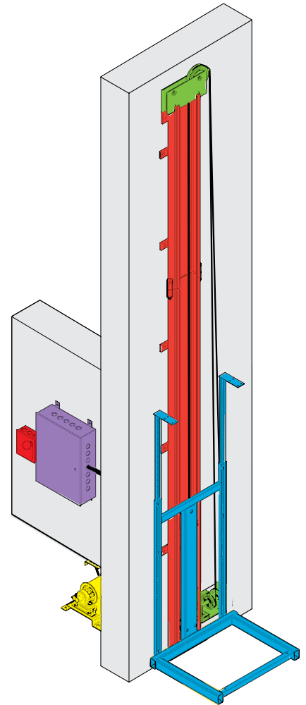
Custom Lift - Winding Drum Series 210 - Capacity 500 lbs
