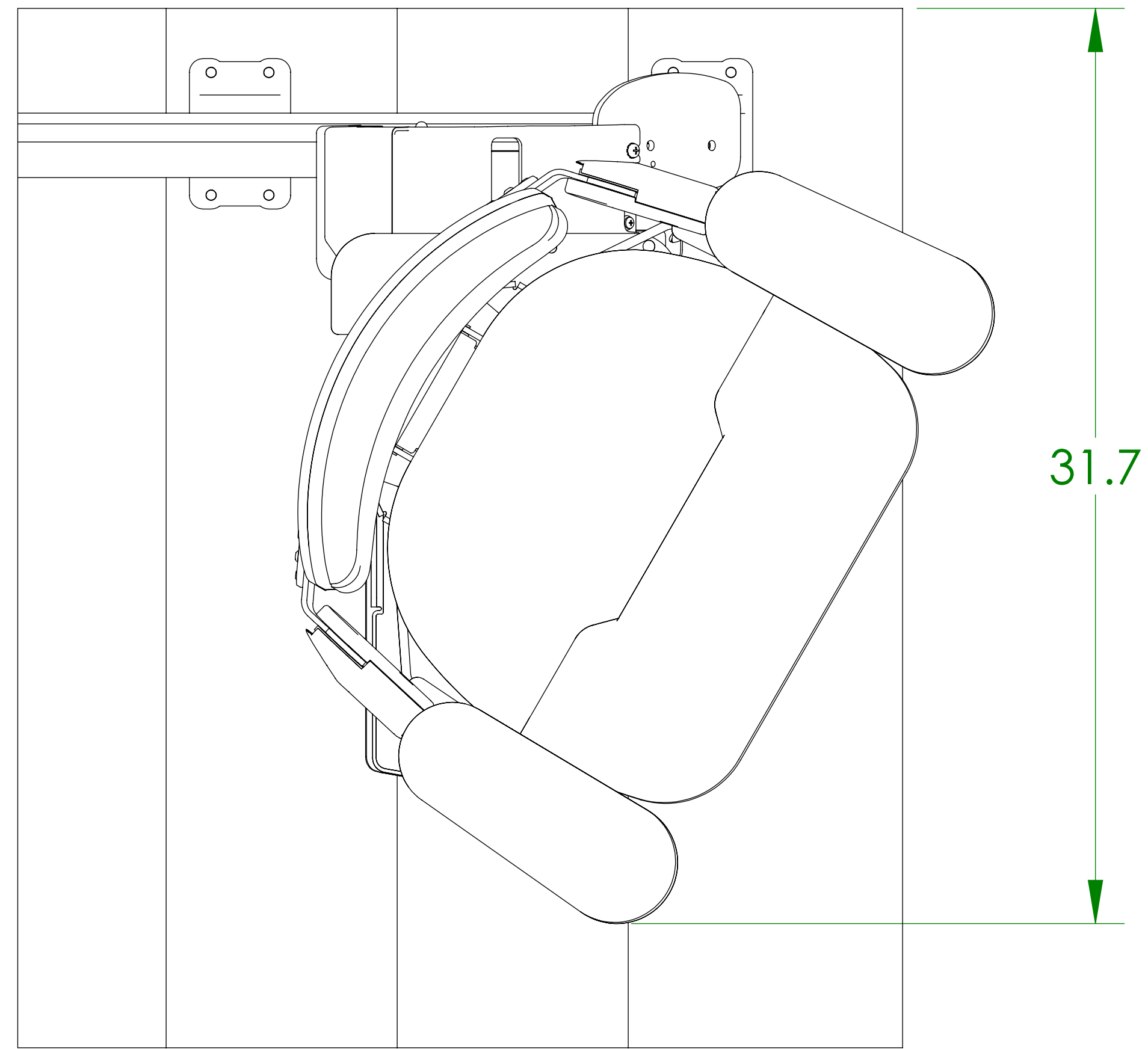
SEAT SWIVELED 60°
