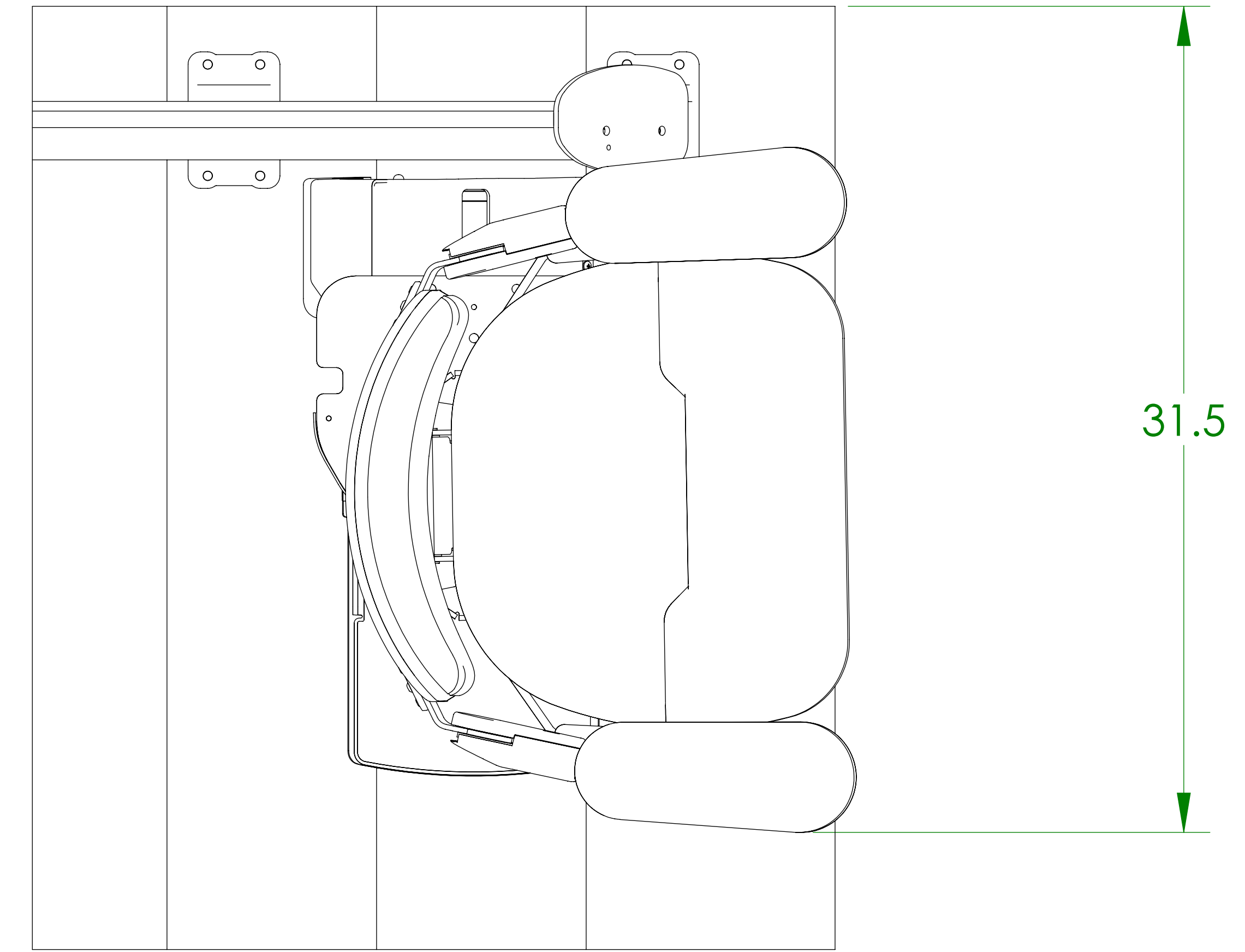
SEAT SWIVELED 90°
