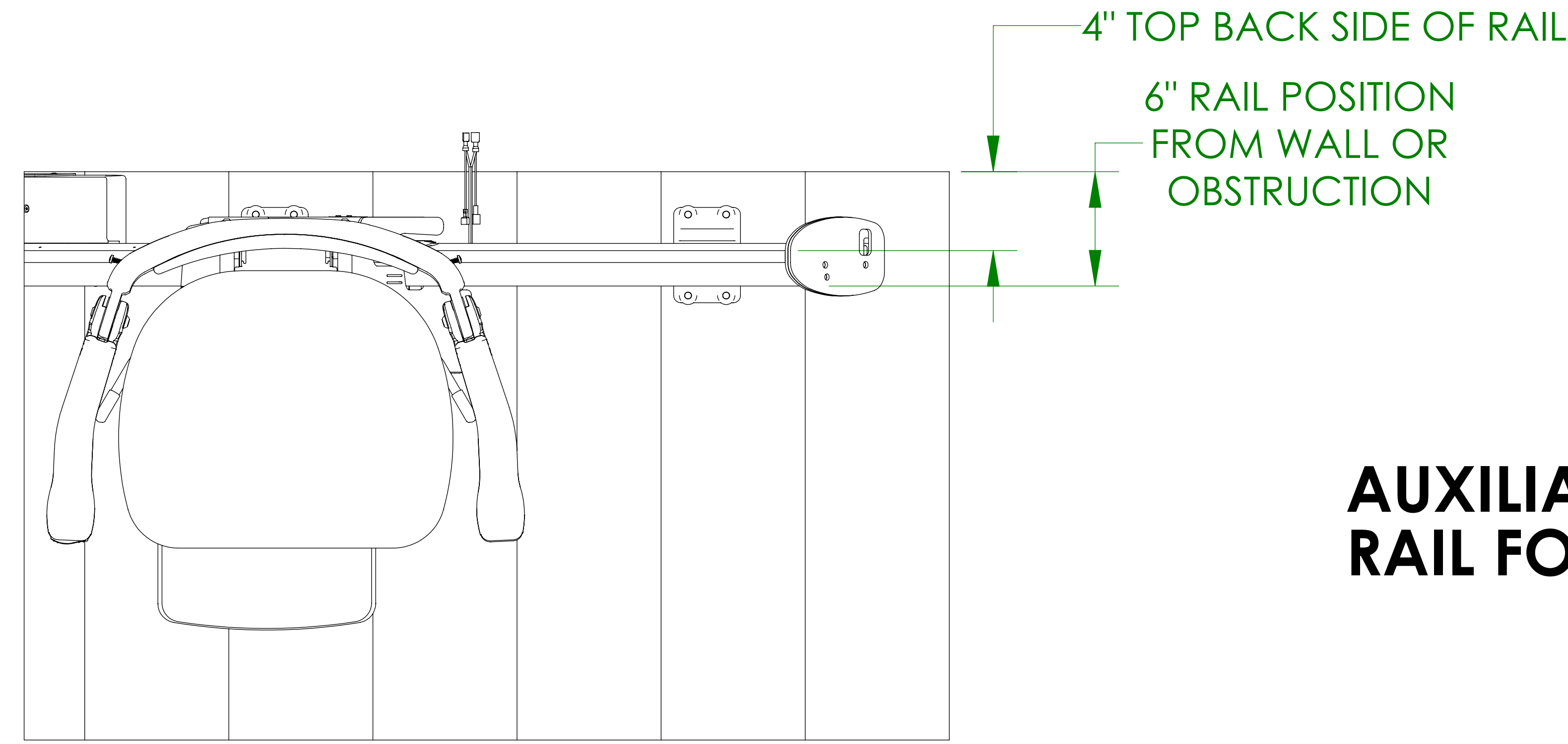
TOP VIEW
